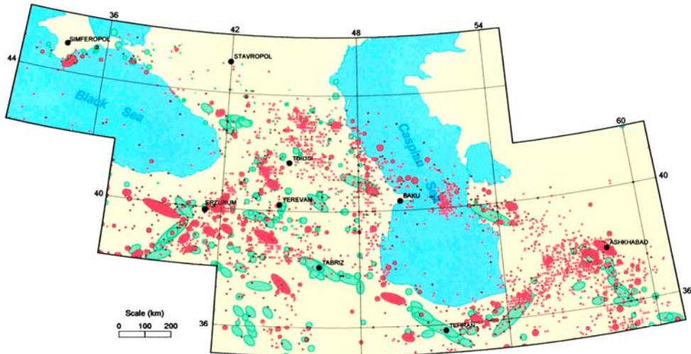
Seismicity of the Caucasus (Balassanian et al, 1999)
